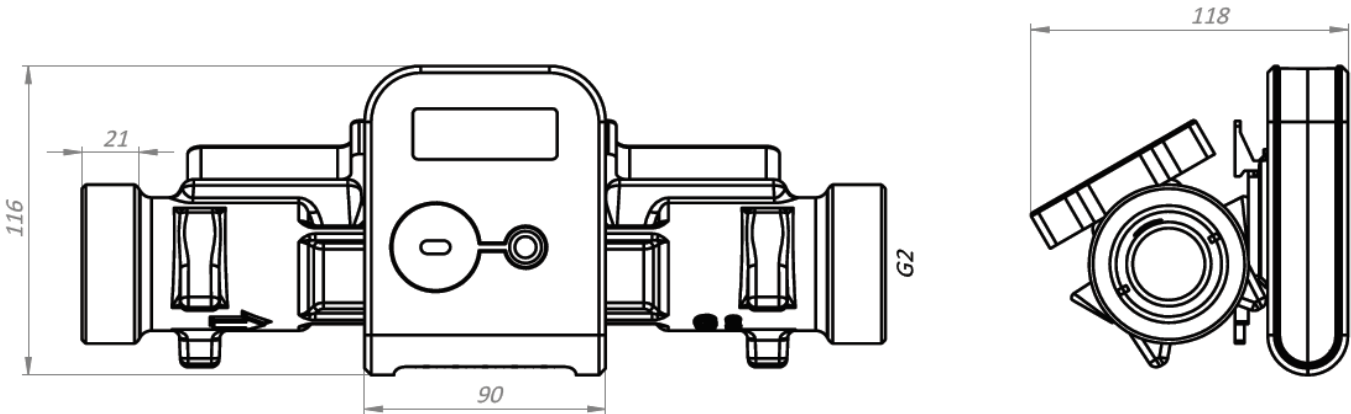
a) connection type: thread G2"
